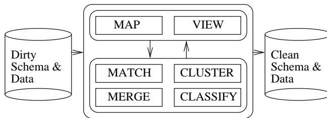
Figure 1: The BIO-AJAX framework.
