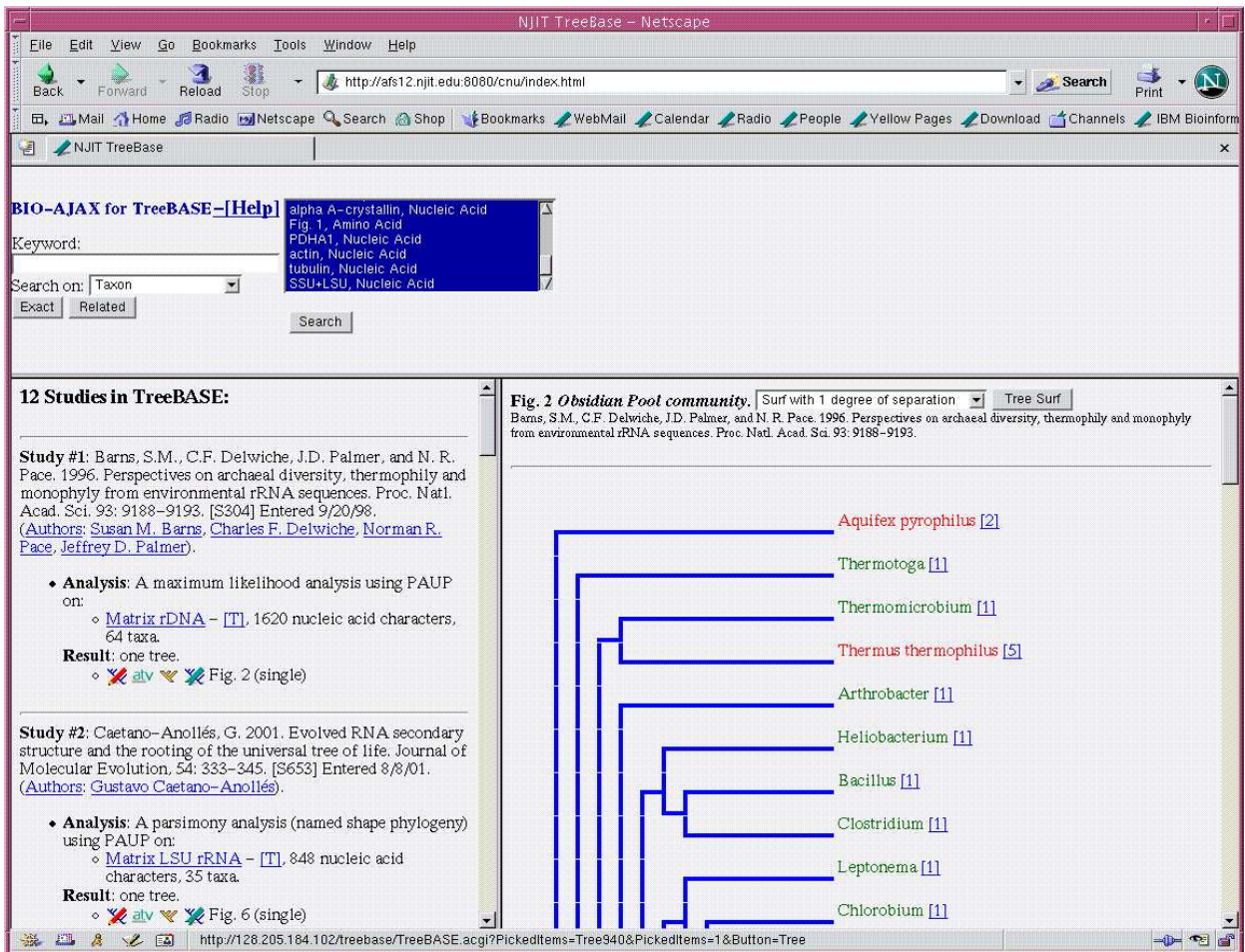
Figure 3: The BIO-AJAX interface implemented for TreeBASE.
